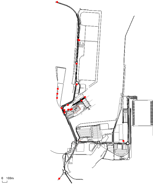
FIGURE 8. Example distribution of 20 sensors obtained with the MILP model.
