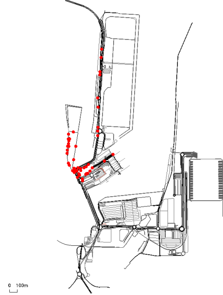
FIGURE 7. Sensor distribution for the best GA solution in Scenario B.
